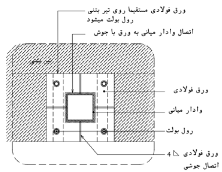
Det.2 sec.C-C
